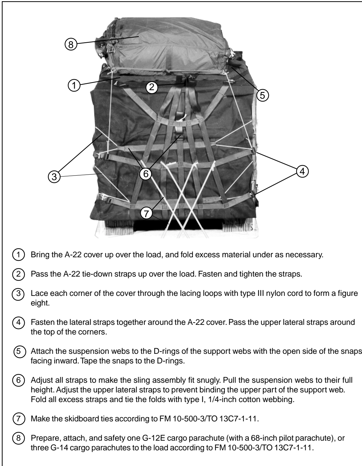
Figure 2-8. A-22 Cargo Bag Secured and Parachutes Installed
